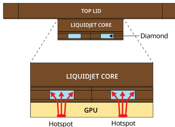
Figure 20: LiquidJet Diamond
