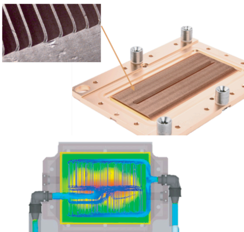
Figure 11: Skived Microchannels in Split-flow coldplate
