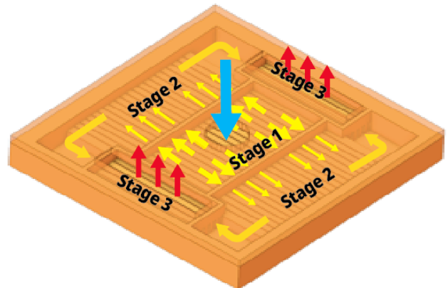
Figure 16: Coldplate with multi-stage design
