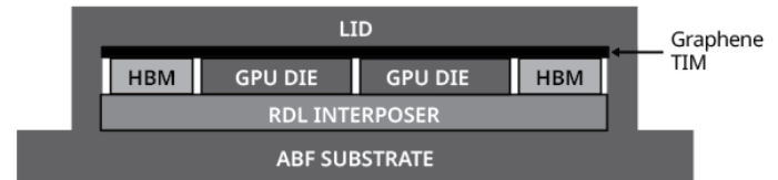
Figure 4: Lidded package design
