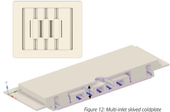
Figure 12: Multi-inlet skived coldplate
