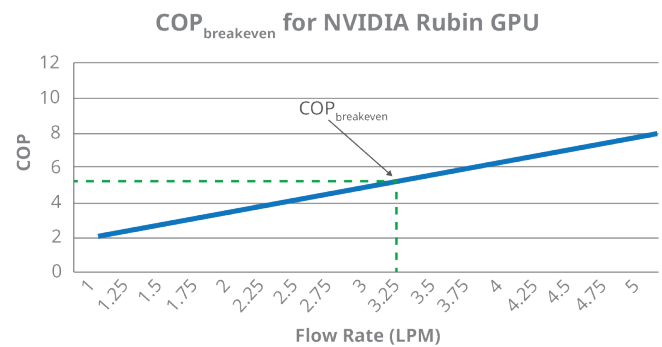
Figure 24: \text{COP}_{\text{breakeven}} for NVIDIA Rubin
