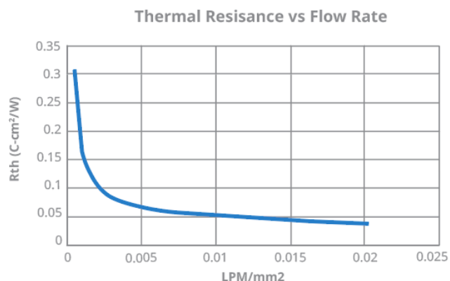
Figure 17: Coldplate thermal resistance vs flow rate for 3D Microcells
