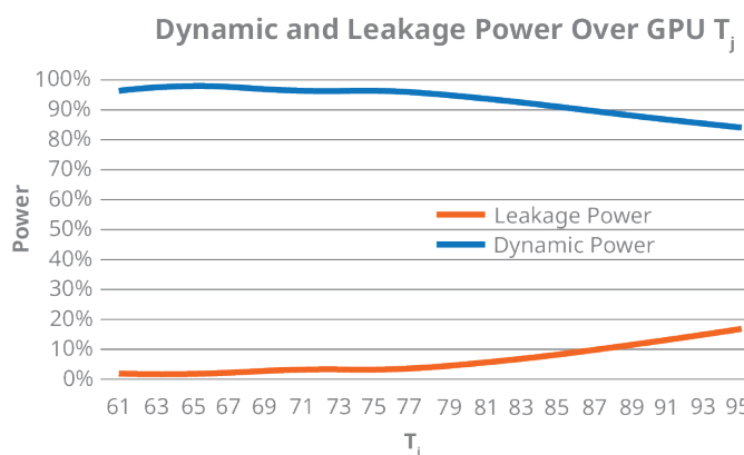
Figure 1: As junction temperature increases, leakage power increases exponentially
