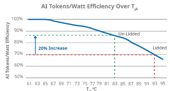
Figure 6: Due to lower thermal resistance, un-lidded packages can achieve higher Tokens/Watt efficiency at the same GPU power by enabling a lower junction temperature
