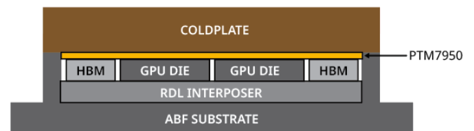
Figure 8: Un-Lidded package design with PTM7950 TIM
