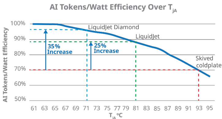
Figure 22: LiquidJet Diamond can achieve higher efficiency at the same GPU power by enabling 10°C lower T_{JA}
