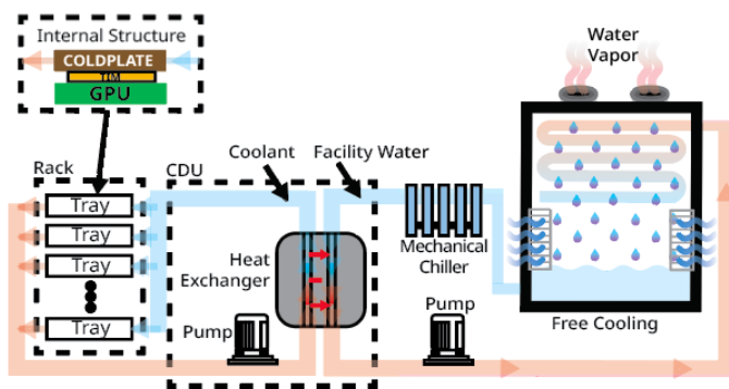
Figure 3: Thermal Stack Components
