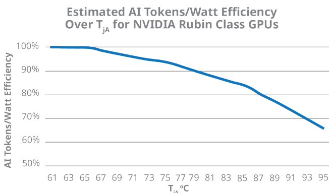
Figure 2: Tokens/Watt efficiency decreases as T_{jA} increases
