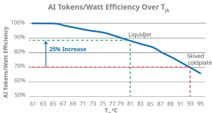
Figure 18: Due to lower thermal resistance, LiquidJet can achieve higher efficiency at the same GPU power by enabling a lower junction temperature
