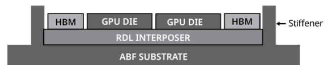
Figure 5: Un-lidded package design
