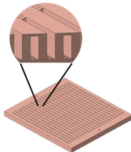
Figure 14: Coldplate with 3D Microcells
