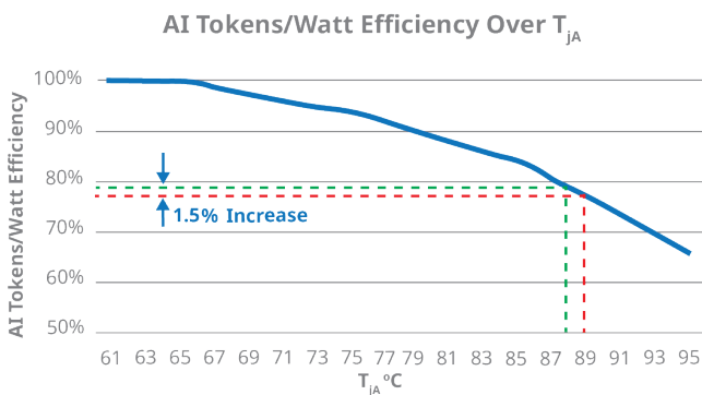
Figure 23: AI Tokens/Watt efficiency 1.5% increase for every 1°C drop in junction temperature
