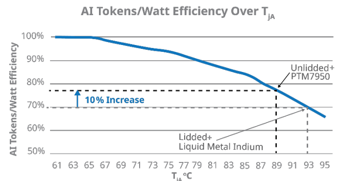
Figure 10: Un-lidded GPU package with PTM7950 TIM delivers higher efficiency at the same GPU power than lidded GPU package with Liquid Metal Indium TIM
