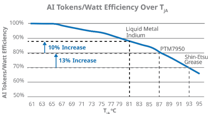
Figure 7: Due to lower thermal resistance, different TIMs can achieve higher efficiency at the same GPU power by enabling a lower junction temperature
