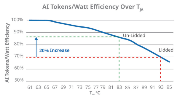
Figure 6: Due to lower thermal resistance, un-lidded packages can achieve higher Tokens/Watt efficiency at the same GPU power by enabling a lower junction temperature
