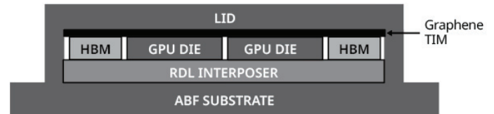
Figure 4: Lidded package design
