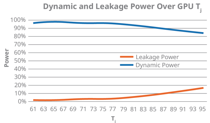
Figure 1: As junction temperature increases, leakage power increases exponentially
