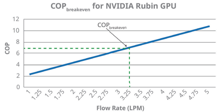
Figure 24: \text{COP}_{\text{breakeven}} for NVIDIA Rubin
