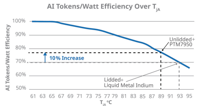
Figure 10: Un-lidded GPU package with PTM7950 TIM delivers higher efficiency at the same GPU power than lidded GPU package with Liquid Metal Indium TIM
