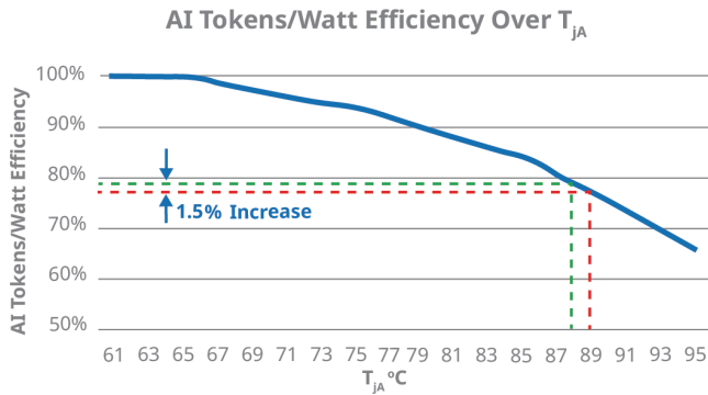
Figure 23: AI Tokens/Watt efficiency 1.5% increase for every 1°C drop in junction temperature
