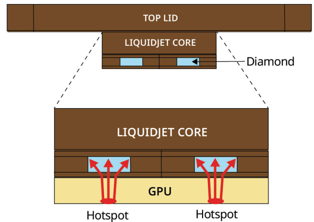
Figure 20: LiquidJet Diamond
