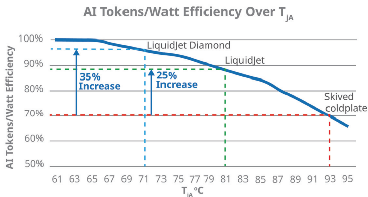
Figure 22: LiquidJet Diamond can achieve higher efficiency at the same GPU power by enabling 10°C lower T_{JA}
