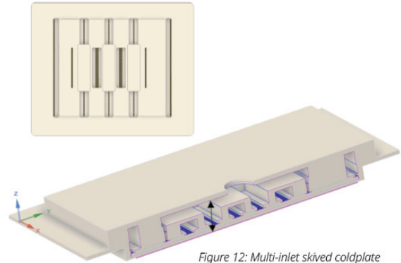
Figure 12: Multi-inlet skived coldplate
